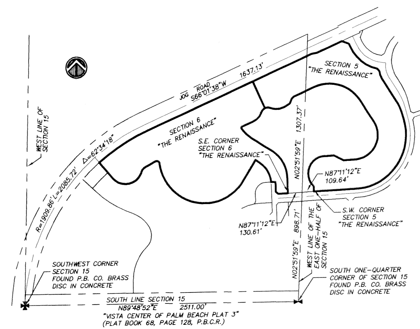
PLAN SHOWING SECTION INFORMATION (NOT TO SCALE)
